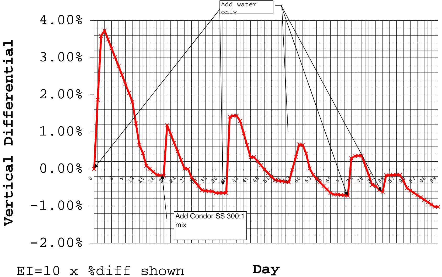
Test #2: Diff. Soil Expansion, 2nd SS Condor Treatment
